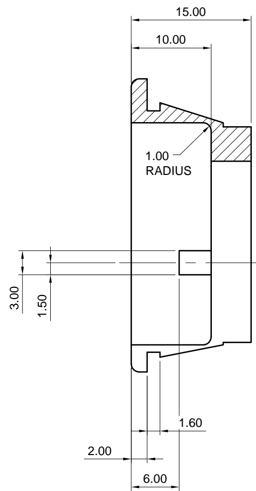
SECTION THRO 'A'-'A'
