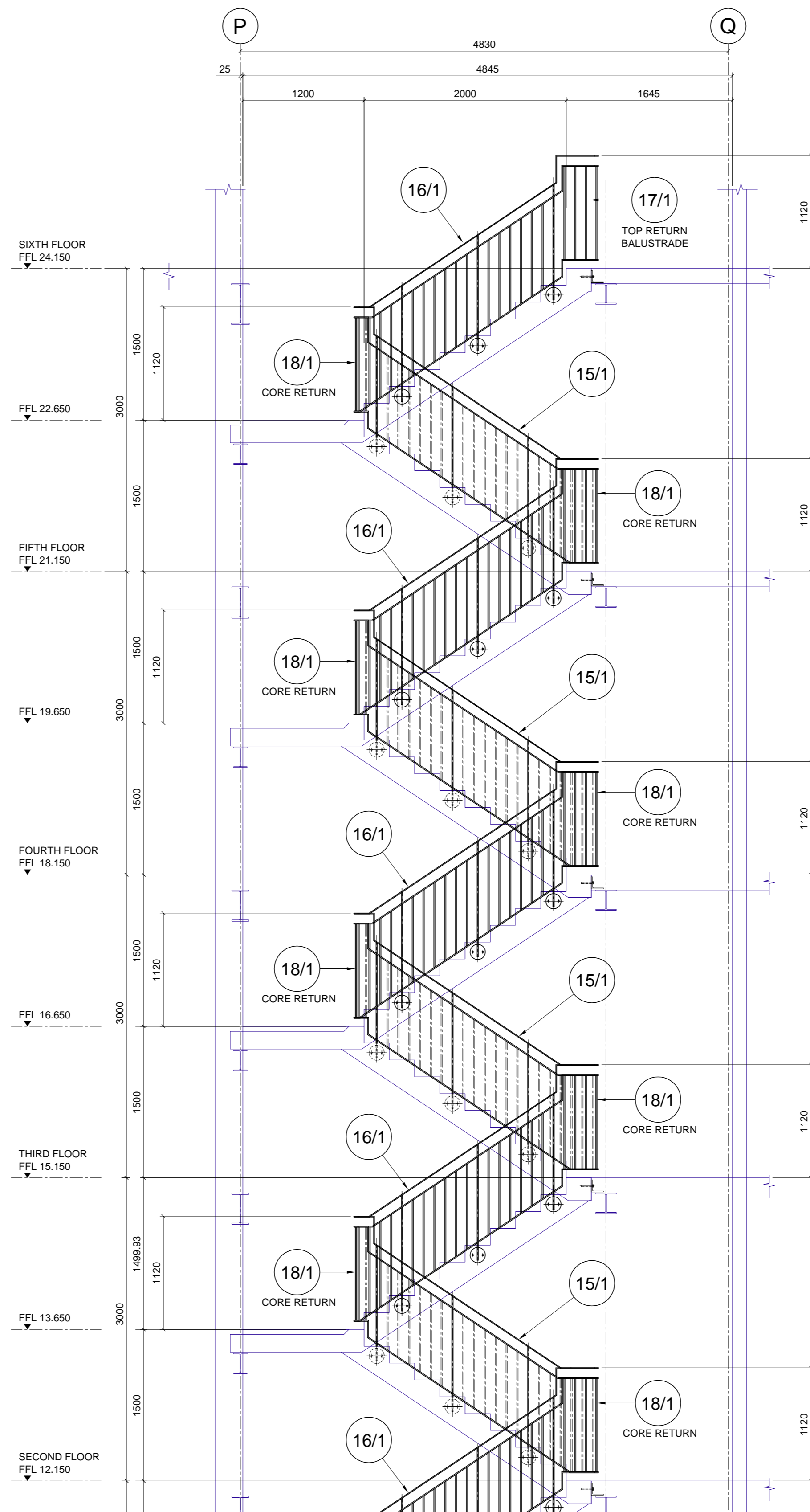
ELEVATION SHOWING BALUSTRADE DETAIL
