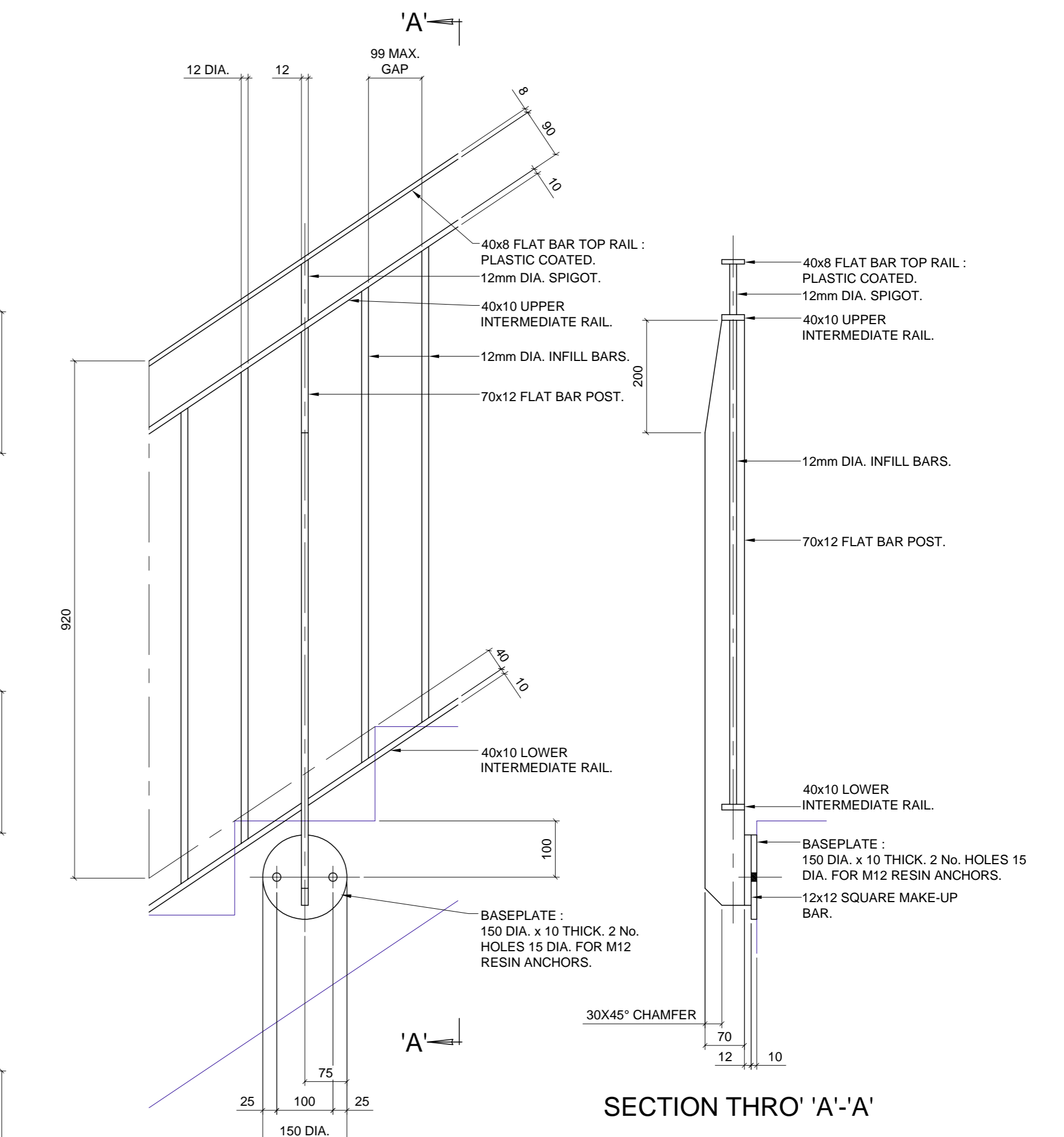
ELEVATION SHOWING BALUSTRADE DETAIL
